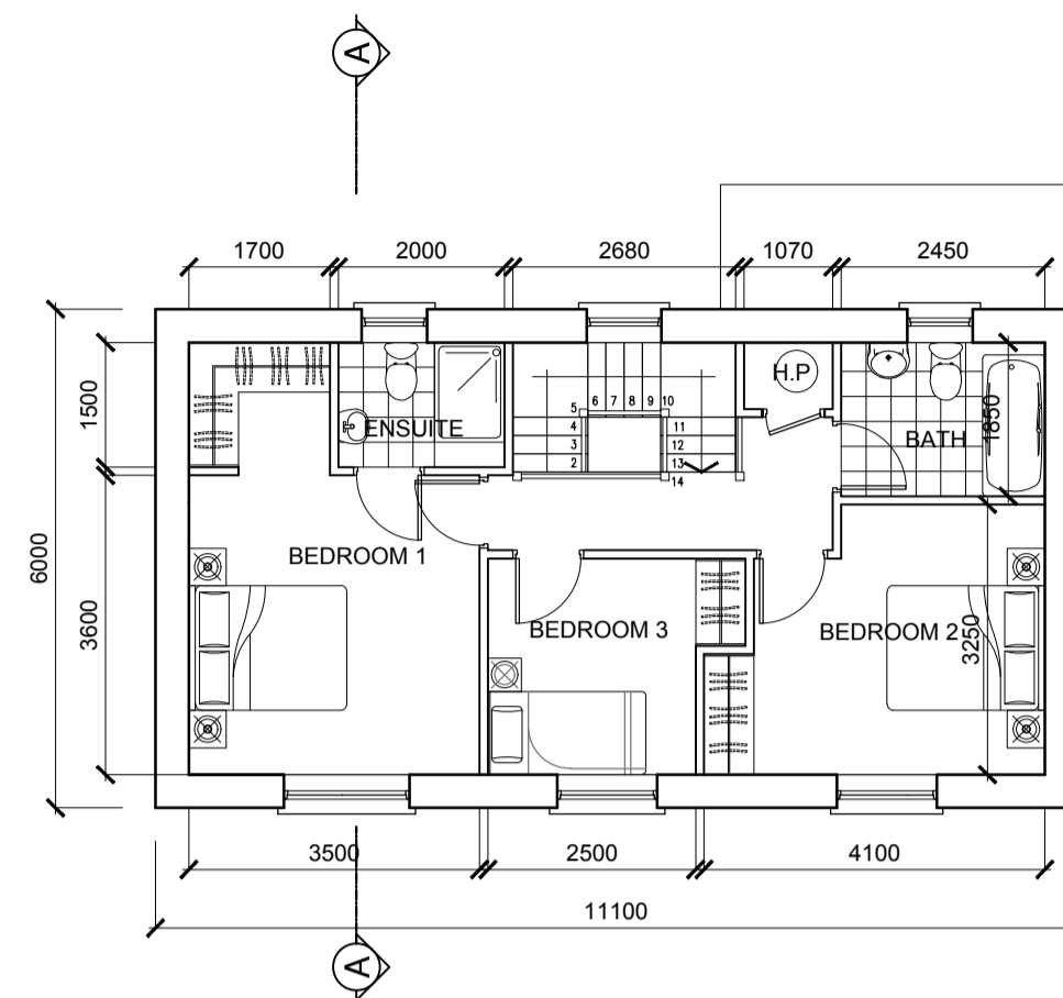
FIRST FLOOR PLAN House Type C - Semi-Detached
