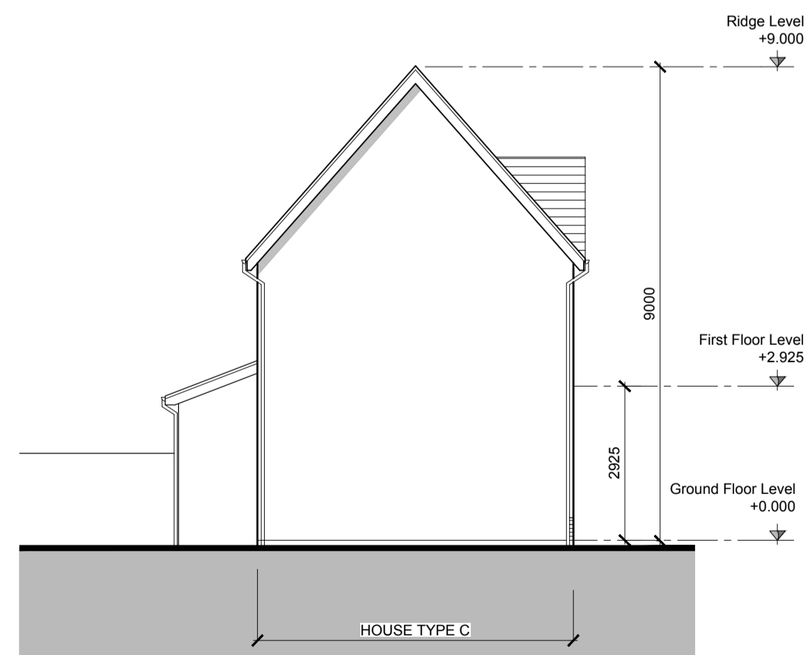
SIDE ELEVATION House Type C - Semi-Detached Left Hand
