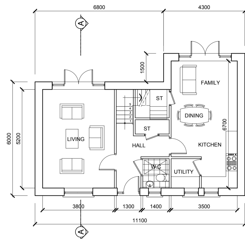
GROUND FLOOR PLAN House Type C - Semi-Detached
