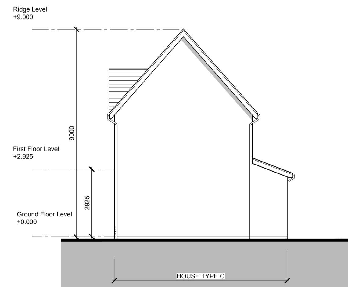
SIDE ELEVATION House Type C - Semi-Detached Right Hand
